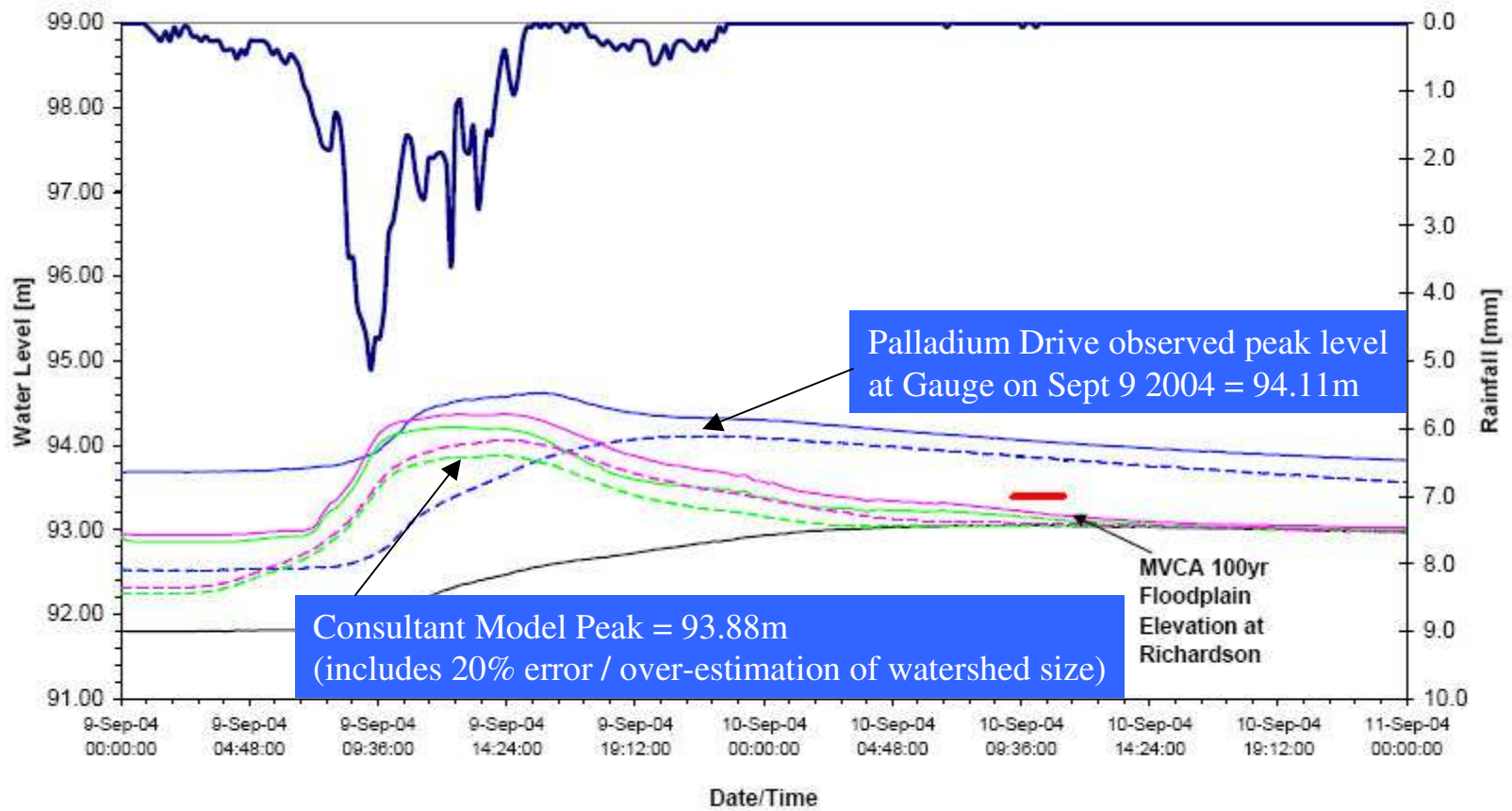
FIGURE 3-3: Carp River - "Hurricane Frances" September 9, 2004 Water Levels (Recorded & Modeled)
